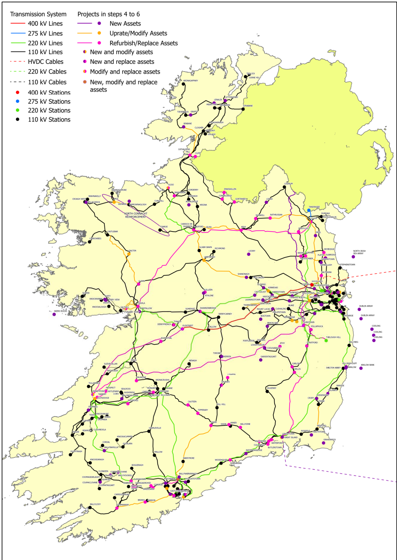
Figure 1-1: All island electricity transmission system (Source: TDP 2023-2032)
